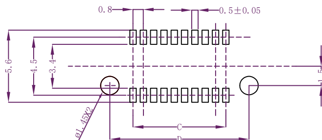
Recommended pc board pattern (TOP VIEW)
