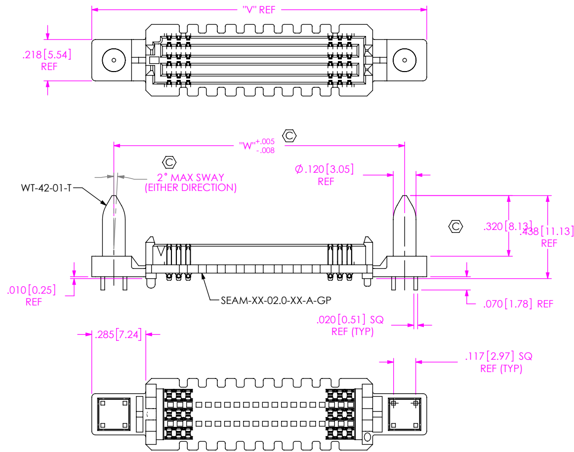
FIG 9 -GP: GUIDE POST OPTION (ONLY AVAILABLE WITH -02.0 LEAD STYLE, 20, 30, 40, & 50 POSITIONS) (MATES WITH SEAF RIGHT ANGLE ONLY) (SEAM-20-02.0-XXX-06-1-A-GP-XR SHOWN) (SAME AS FIG 1, EXCEPT AS SHOWN) (SOME CENTER FEATURES REMOVED FOR CLARITY)
