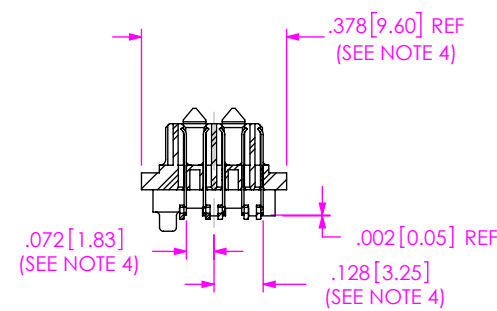
SECTION "G"-"G" FIG 7 -05: 5 ROWS (SEAM-20-03.5-XXX-05-1-A-XR SHOWN) (SAME AS FIG 6, EXCEPT AS SHOWN) (SOME CENTER FEATURES REMOVED FOR CLARITY) (SEE NOTE 4)
